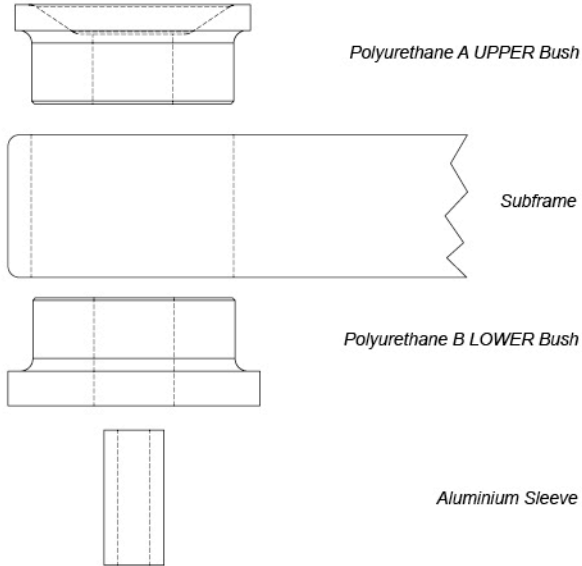
Figure 1: Exploded Diagram
