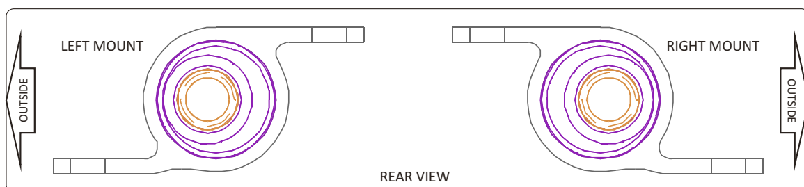
Fig 3. Maximum positive caster setting.
