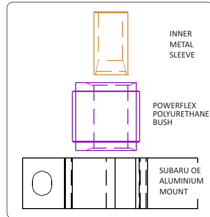
Fig 1. Exploded view.
