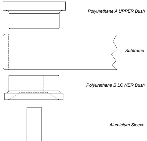
Figure 1: Exploded Diagram
