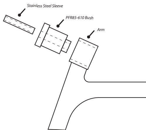
Figure 1: 6R0 Part number fitting
